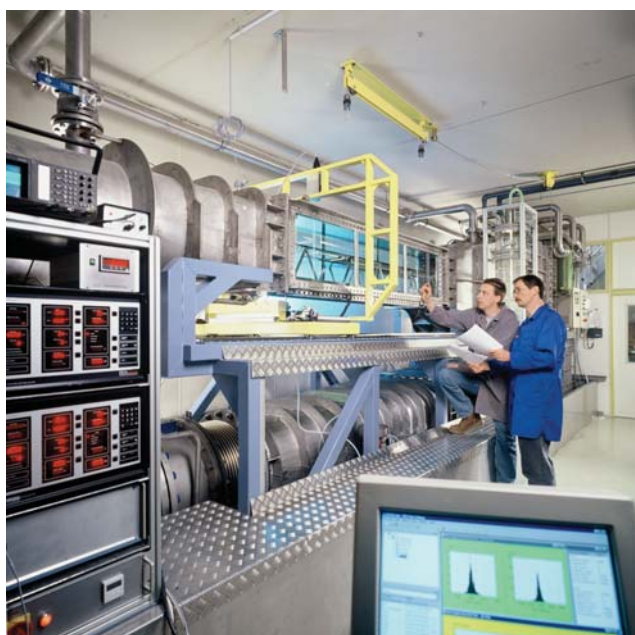
FIGURE 2 MATCHED-INDEX-OF-REFRACTION TUNNEL AT UNI. ERLANGEN
